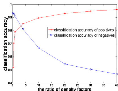
Figure 1. Classification accuracy with different r_1 / r_2 ratio.
